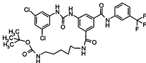
Compound # 5
